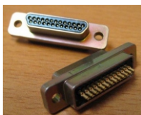
25-way Microminiature-D Plug with pins
